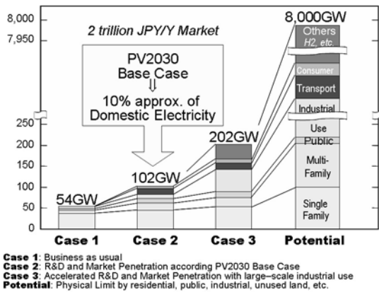
Fig. 4 Installable PV (GW) assuming Technological Progresses up to 2030
