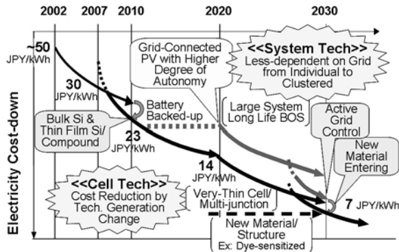
Fig. 5 Cost-down Scenario toward 2030
