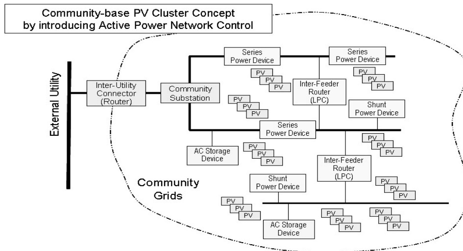
Fig. 8 A basic network image of “Autonomy-Enhanced PV Clusters” by utilising power electronic devices and battery storage stations
